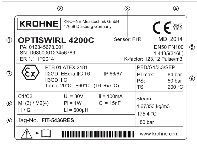
Figure 2-8: Example of nameplate
