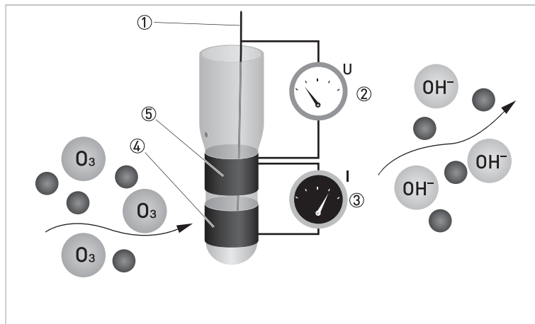
Figure 1-4: Ozone measurement
