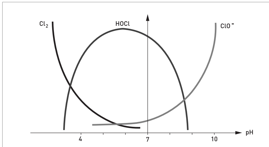
Figure 1-2: Composition of free chlorine depending on pH value
