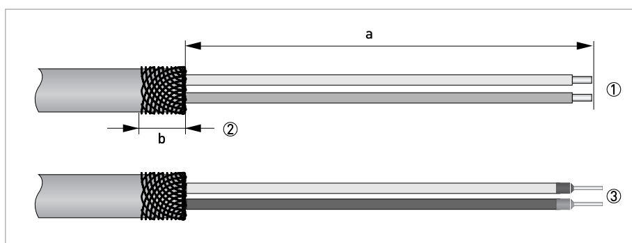
Figure 3-7: Preparation of field current cable C
