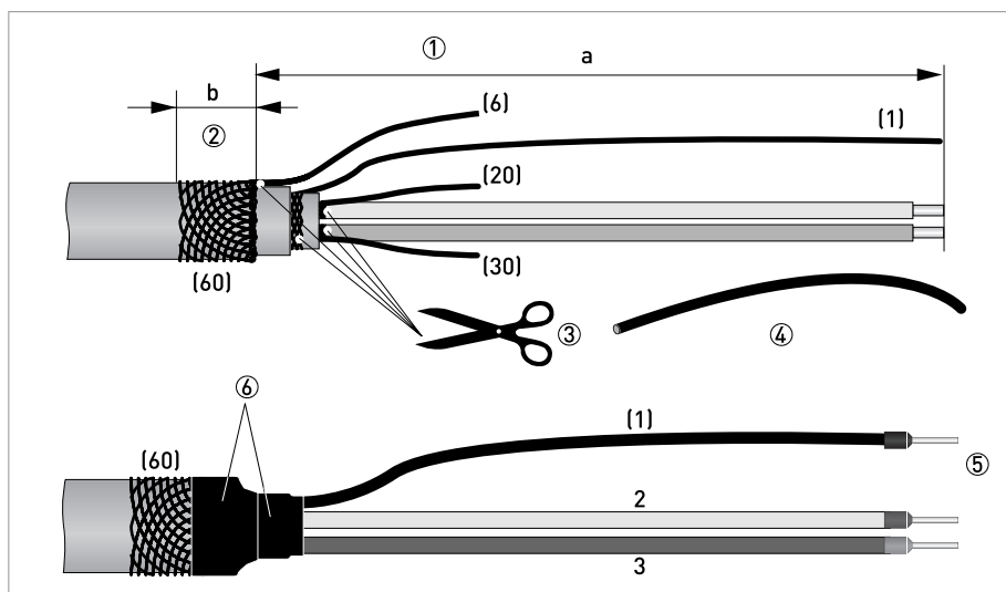
Figure 3-6: Preparing signal cable B, connection to measuring sensor
