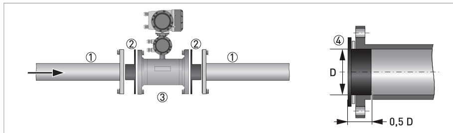
Figure 3-11: Grounding with grounding rings
