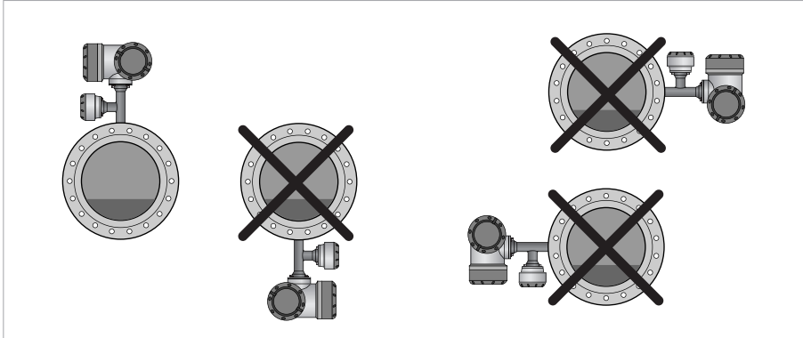
Figure 2-13: Mounting position
