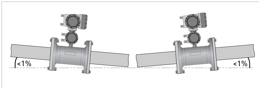
Figure 2-8: Recommended slope
