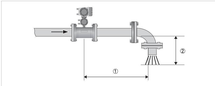
Figure 2-10: Open discharge
