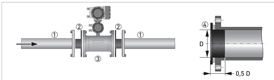
Figure 2-14: Grounding with grounding rings
