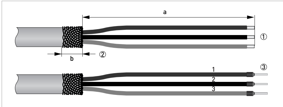
Figure 3-8: Preparing the interface cable
