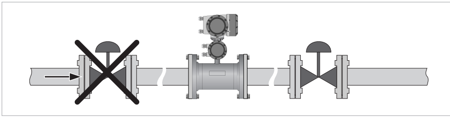
Figure 2-7: Installation before control valve
