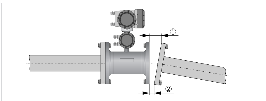
Figure 2-12: Flange deviation
