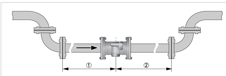
Figure 2-6: Recommended inlet and outlet sections, top view
