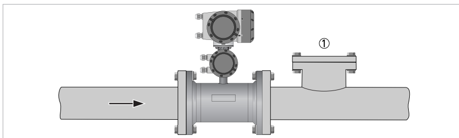
Figure 2-11: Option for cleaning of flow sensor
